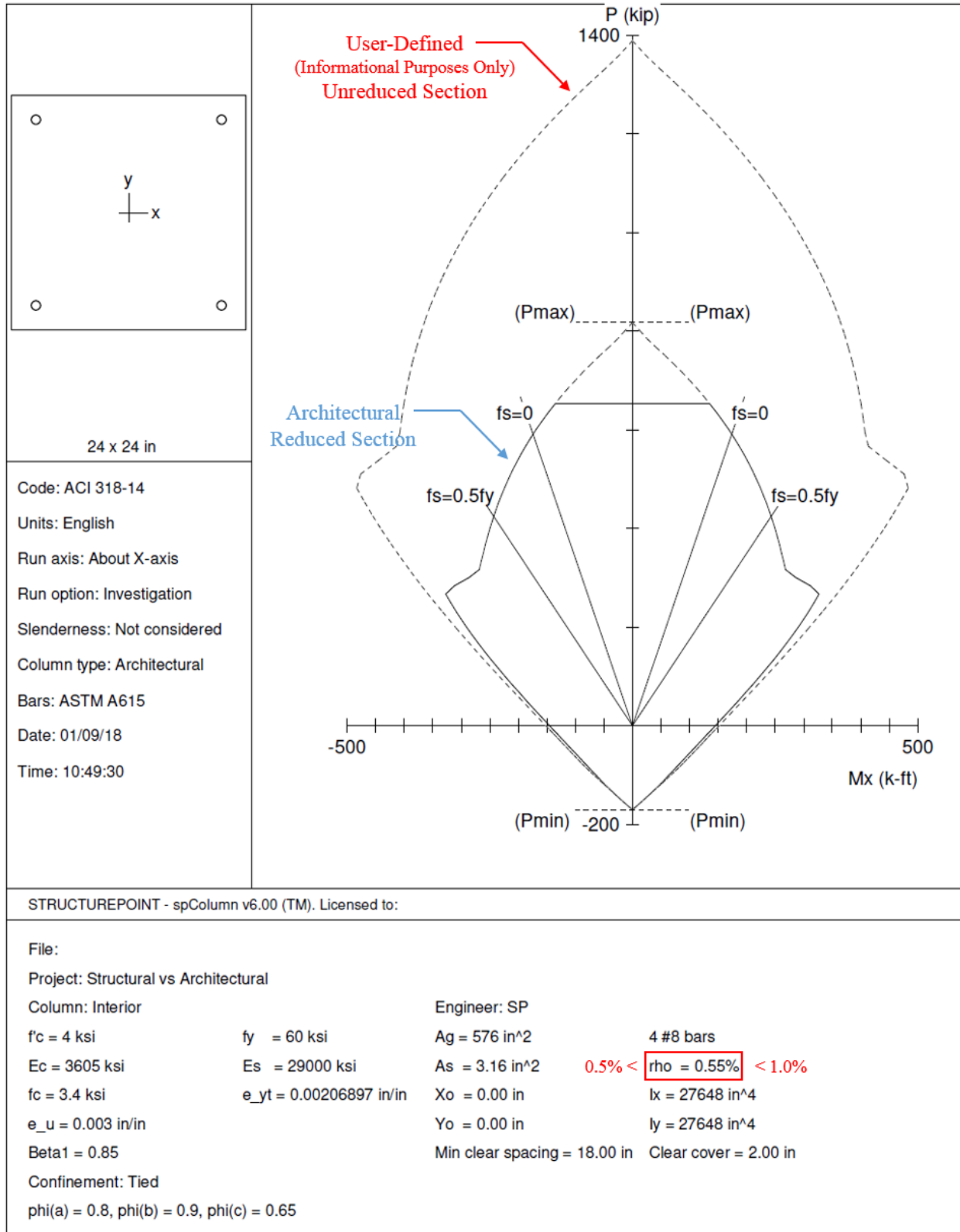
Figure 3 – Superimposed architectural and user-defined factored column interaction diagrams
